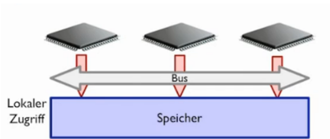
Abbildung 5: SMP (Symmetric Multi Processing)
